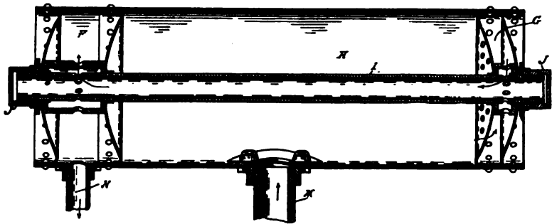
HARRINGTON PERFORATED BAFFLE PLATE MUFFLER.
